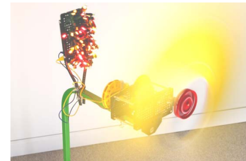
A student designed TeacherGeek Wind Turbine using an Alternator to power over 100 lights.
